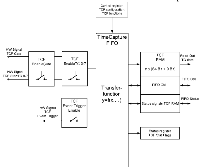
Fig. 3: Structure of the TCF device
