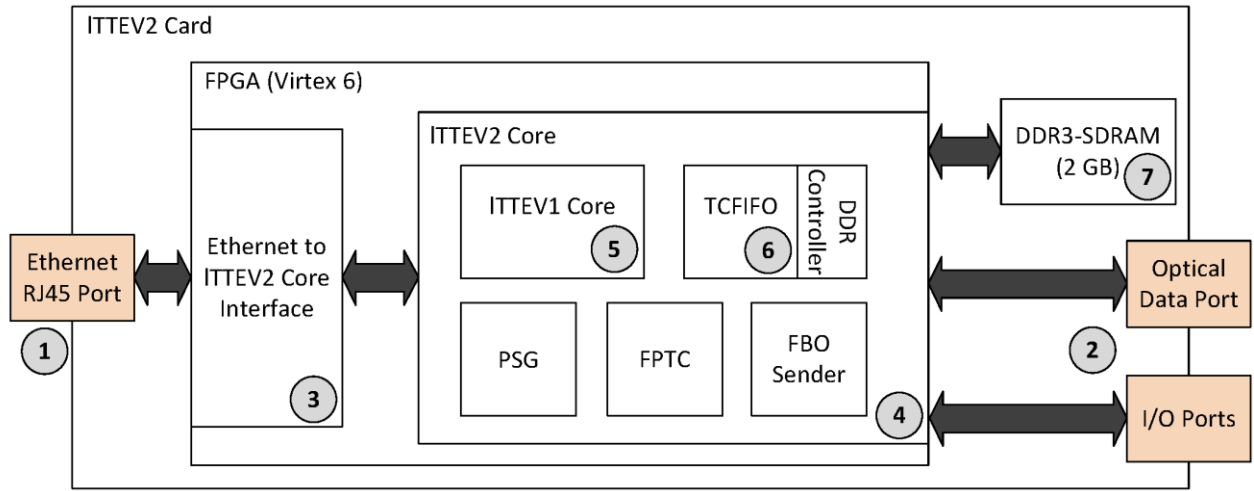
Fig. 1: System architecture of the ITTEV2 card
