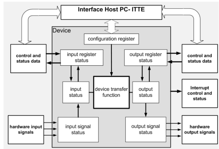
Fig. 1: Generic model of a TTE device
