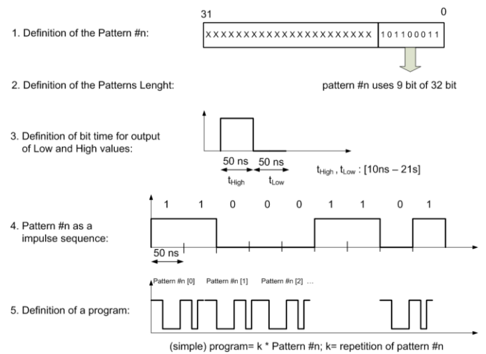
Fig. 4: Definition of a simple impulse program consisting of one pattern
