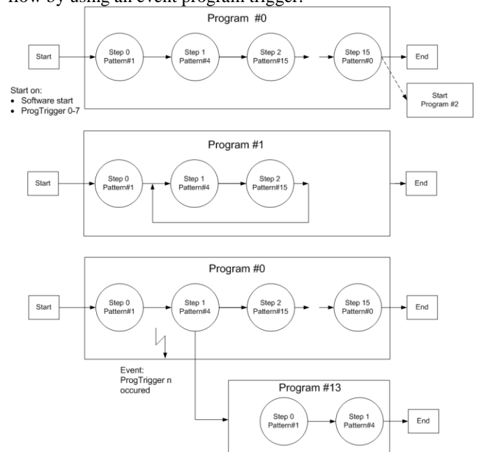
Fig. 5: Program examples for pulse sequences of a PSG
