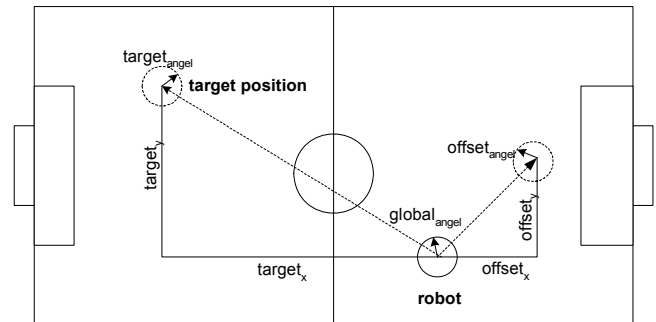
Fig. 9. An example configuration for the slip and friction compensation. For details please see text.
