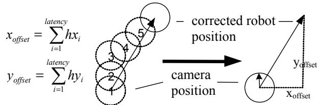
Fig. 7. Extrapolation of the robot's position using the image processing system and the robot's previous tick count.
