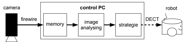
Fig. 2. The image processing system consists of five stages which all contribute to processing delays also known as latency time.
