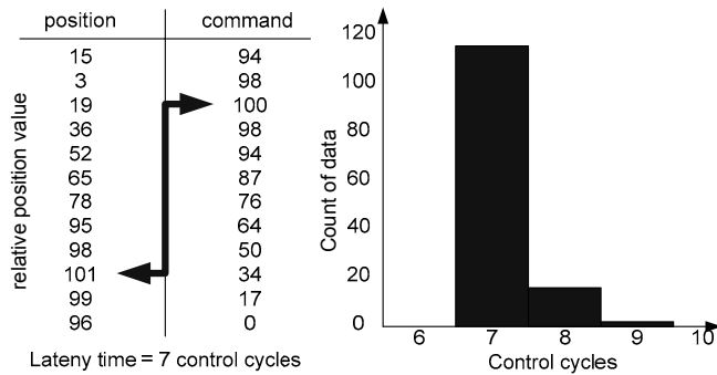
Fig. 6. Detection of the Latency time in the control loop.
