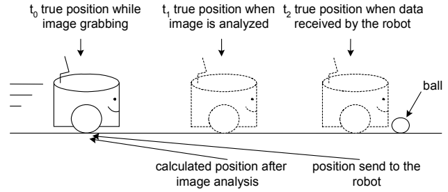
Fig. 4. Due to the latency problem, the robot receives its commands at time t_2 , which actually correspond to the image at time t_0 .
